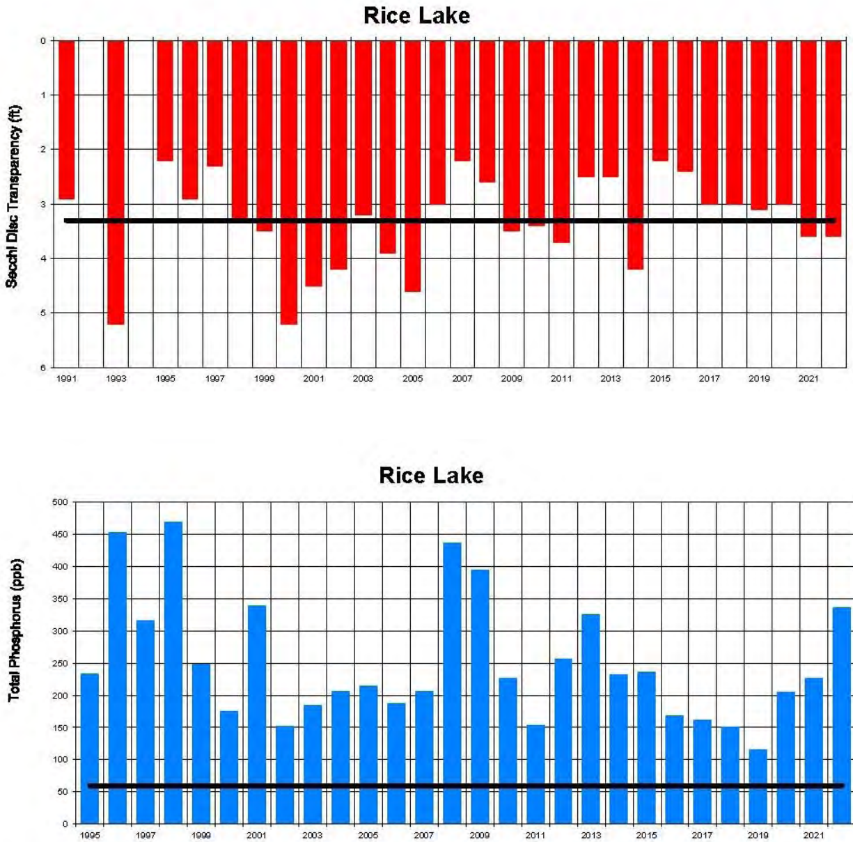
Figure 1. Seasonal averages (May - September) for Secchi disc transparency (top) and total phosphorus (bottom). Recent fish surveys have been conducted in 2008, 2014, 2022, and 2023. The black line indicates the threshold for impaired or unimpaired water quality. For Secchi disc transparency, values greater than 3.3 feet are unimpaired. For phosphorus, concentrations less than 60 ppb are unimpaired.
